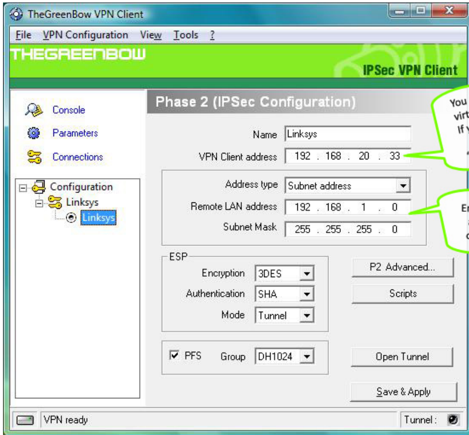
Phase 2 Configuration
